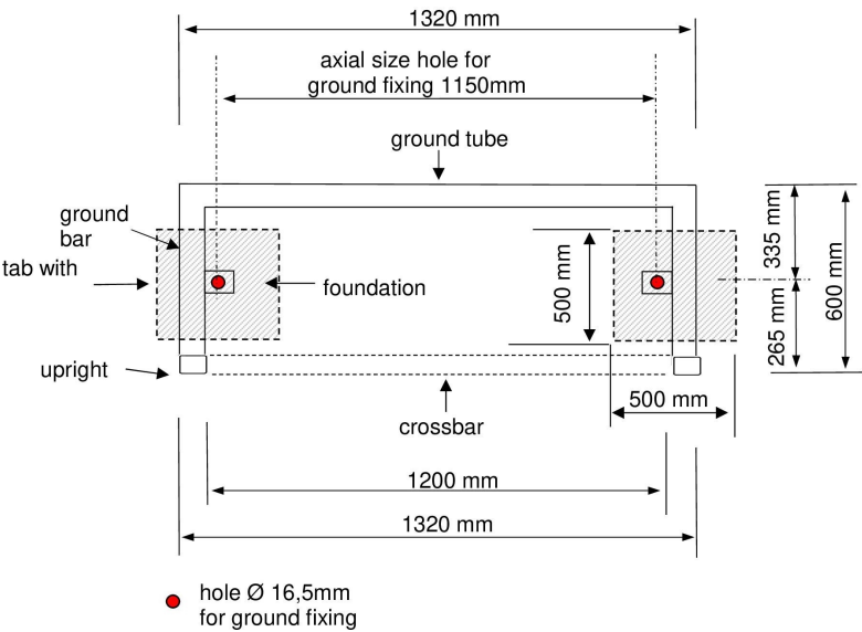
Example foundation drawing:
