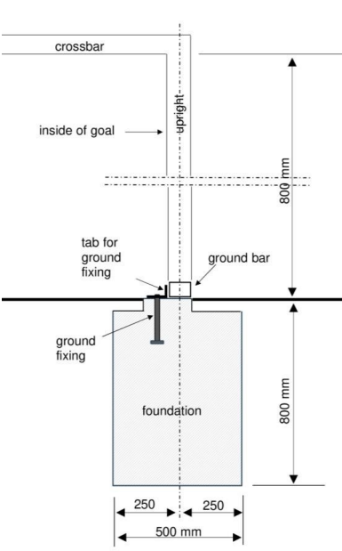
Exmample 2 foundation section B-B
