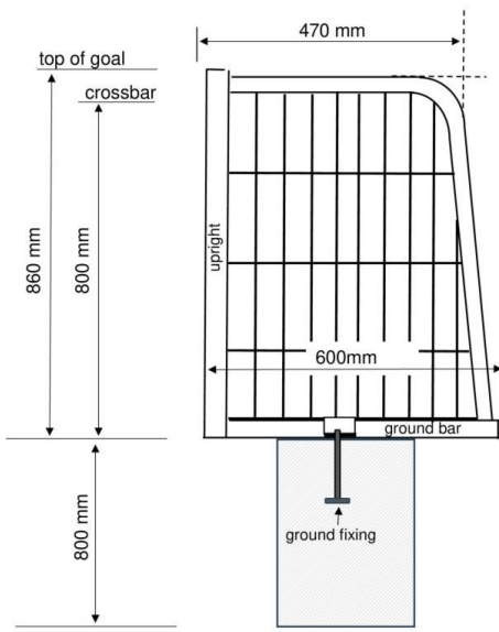
Example foundation section A-A:
