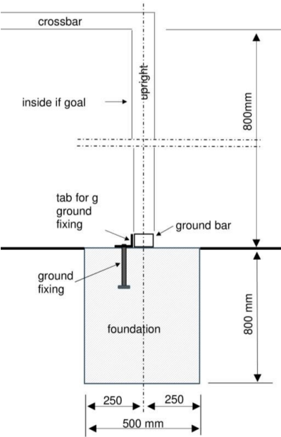
Exmample 1 foundation section B-B
