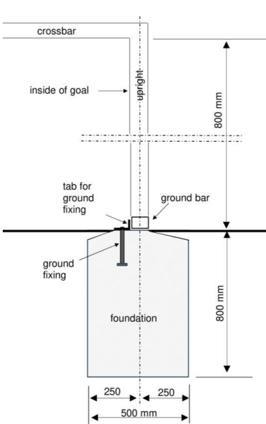
Exmample 3 foundation section B-B
